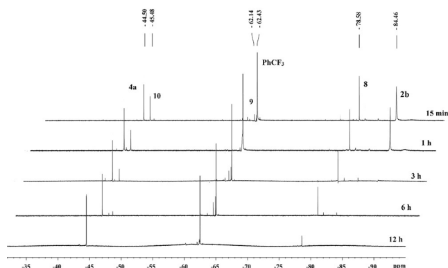
Figure 2. Progress of the reaction of 3a , for up to 12 h, by ^{19}\text{F} NMR spectroscopy. The peaks (in \text{CDCl}_3 ) represent \text{CF}_3\text{SO}_2\text{Na} ( 2b , \delta = -84.46 ppm), \text{CF}_3\text{S}(\text{O})\text{H} ( 8 , \delta = -78.58 ppm), the internal standard ( \text{PhCF}_3 , \delta = -62.43 ppm), \text{CF}_3\text{S}-\text{OH} ( 9 , \delta = -62.14 ppm), \text{CF}_3\text{SSCF}_3 ( 10 , \delta = -45.48 ppm), and 4a ( \delta = -44.50 ppm).
