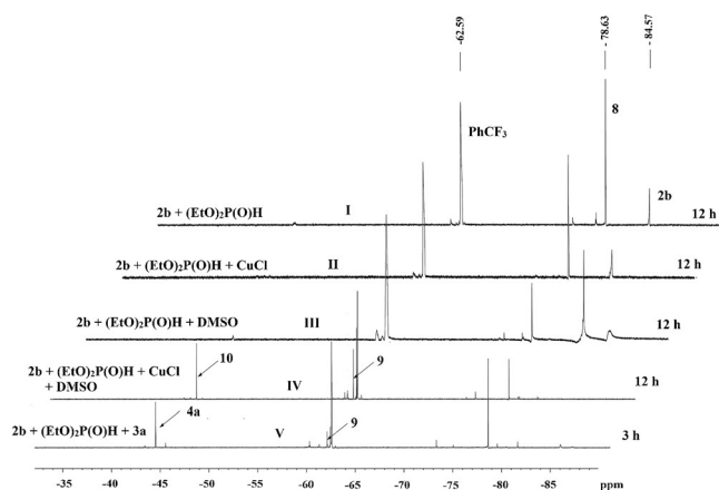
Figure 3. Progress of reactions without indole, at 110^\circ\text{C} , using ^{19}\text{F} NMR (in \text{CDCl}_3 ) spectroscopy.
