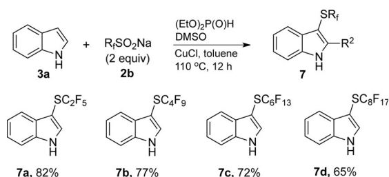
Scheme 2. Perfluoroalkylthiolation of indole. Reaction conditions: 3a (0.2 mmol), R_f\text{SO}_2\text{Na} (0.4 mmol), (\text{EtO})_2\text{P}(\text{O})\text{H} (0.4 mmol), DMSO (0.6 mmol), CuCl (0.2 mmol) in PhMe (1 mL) under \text{N}_2 at 110^\circ\text{C} for 12 h. Yields are those of the isolated products.
