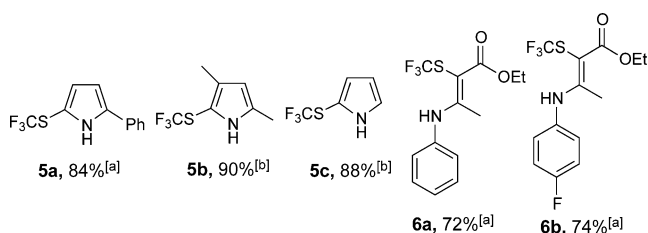
Scheme 1. Trifluoromethylthiolation of pyrroles and enamines. Reaction conditions: pyrroles or enamines (0.2 mmol), 2b (0.4 mmol), (\text{EtO})_2\text{P}(\text{O})\text{H} (0.4 mmol), DMSO (0.6 mmol), CuCl (0.2 mmol) in PhMe (1 mL) under \text{N}_2 at 110 °C for 12 h. [a] Yield of isolated product. [b] Yield determined by GC-MS.
