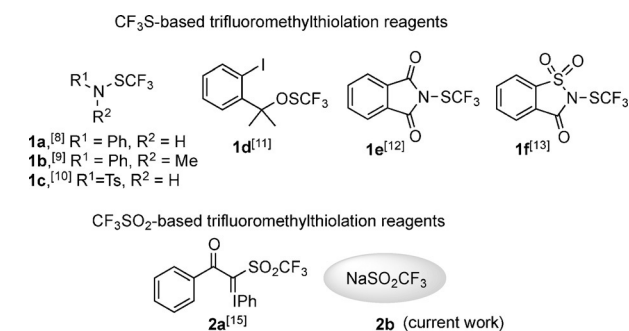
Figure 1. User-friendly trifluoromethylthiolation agents. Ts = 4-toluene-sulfonyl.
