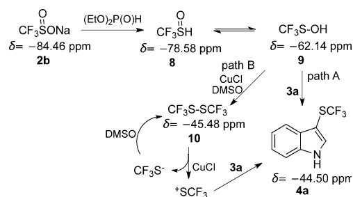
Scheme 3. Proposed mechanism for \text{CF}_3\text{SO}_2\text{Na} trifluoromethylthiolation.
